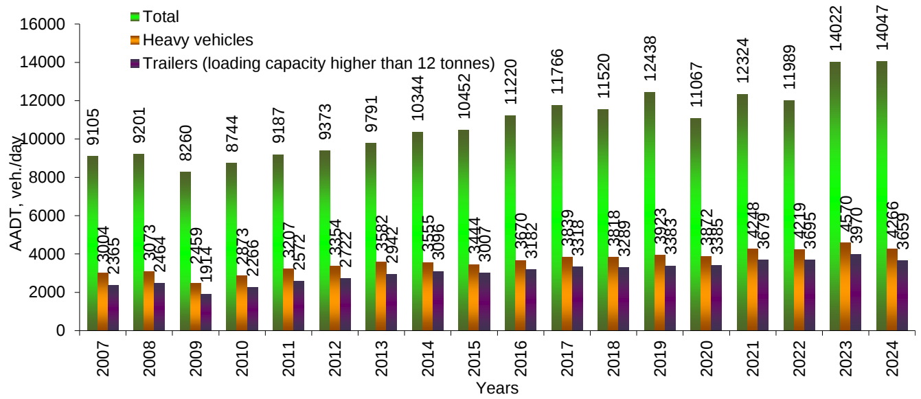
Change of annual average daily traffic (AADT) on the transport corridor Via Baltica since 2007
